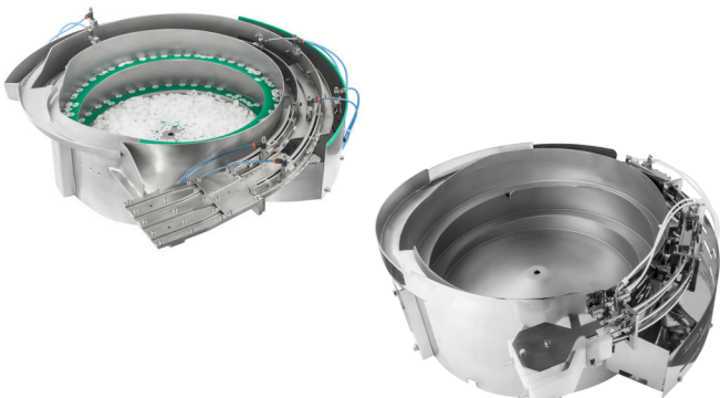
HIGH PERFORMANCE BOWL FEEDERS CI AND TC FROM 160 TO 900 MM DIAMETER
