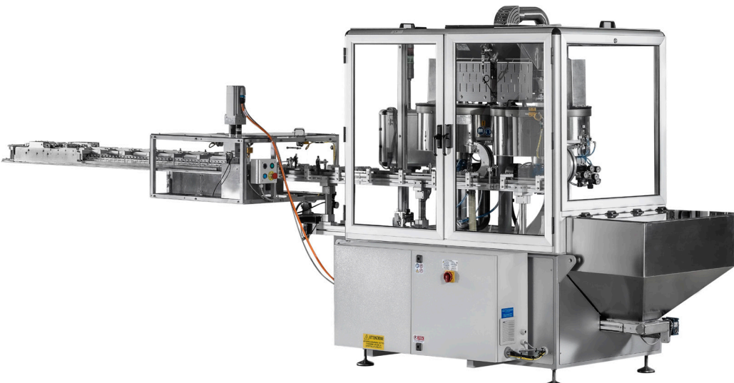
HIGHSPEED PRECISION FEEDINGSYTEM RR INLINE FEEDER FOR MULTIPLE (E.G. 16) TAKE-OVER POSITIONS
