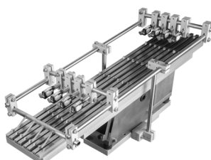
CONVEYORS: JETSTREAM/ BELT CONVEYORS/VIBRATORY/ CHUTES
